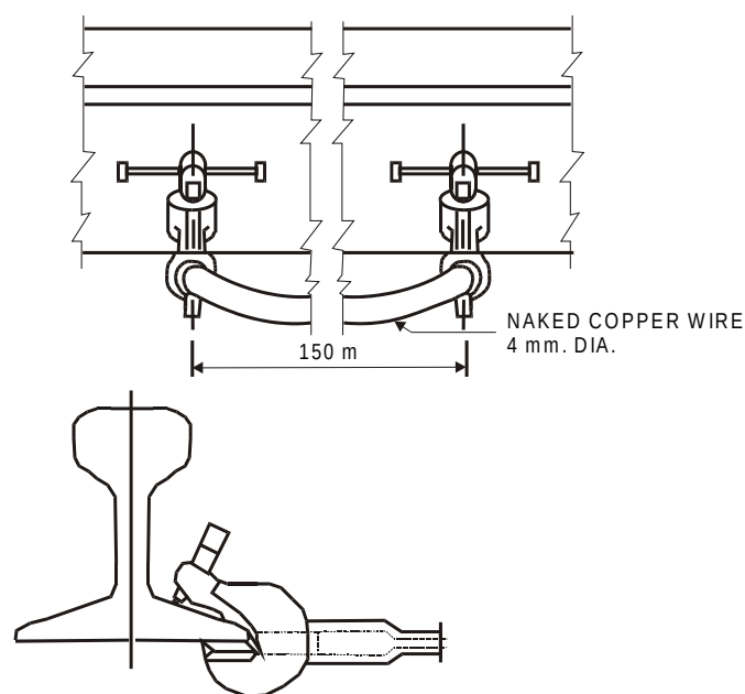
TEMPORARY JUMPERING OF RAILS IN CASE OF RAIL FRACTURES
