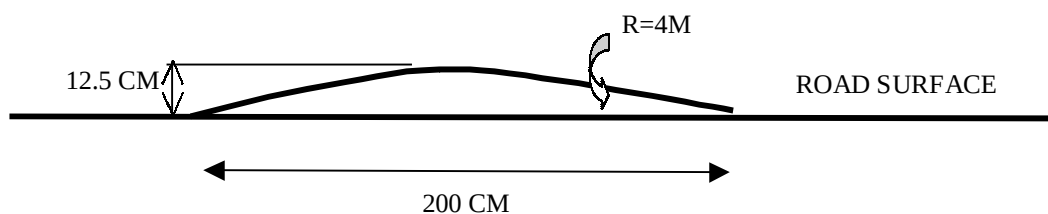
SPEED BREAKER – SECTION –‘AA’
