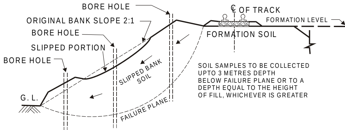
CROSS SECTION SHOWING SAMPLING LOCATIONS ON SLIPS OF BANKS
