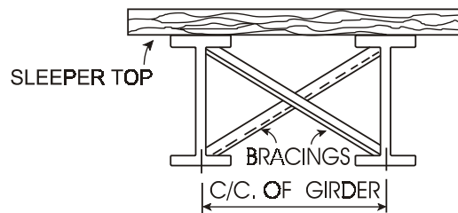
FIG. 1 MAKING RAIL SEATS IN ONE PLANE
