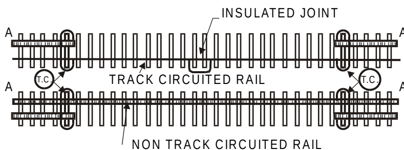
3) REMOVING OF ONE RAIL (ONE RAIL ONLY INSULATED FOR TRACK CIRCUITING)
