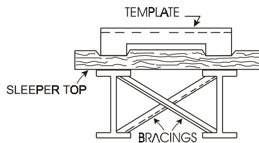
FIG. 4: CHECKING OF NOTCHED SURFACES TO BE IN ONE PLANE
