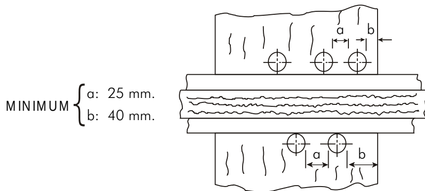
IN SITU PLUGGING AND REBORING OF HOLES
