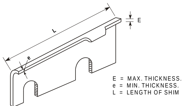
SKETCH SHOWING THE TAPERED SHIM IN USE
