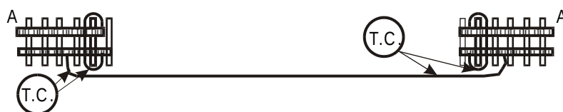
2) REMOVING BOTH THE RAILS, SIMULTANEOUSLY OF ONE LINE (BOTH THE RAILS INSULATED FOR TRACK CIRCUITING)
