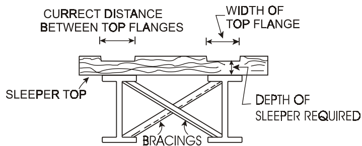
FIG. 2: MAKING OF NOTCHES FOR SEATING ON GIRDER FLANGES
