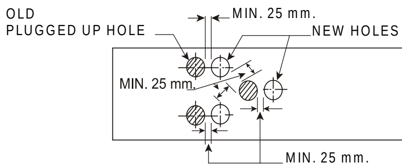
PLUGGING AND REBORING OF WOODEN SLEEPERS AT THE TIME OF RECONDITIONING
